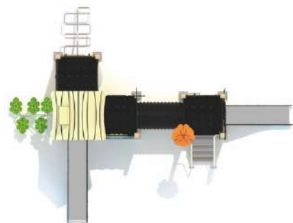
GW-03602 UNIT SIZE: 680*500*410 CM SAFETY ZONE 1050*870 CM
